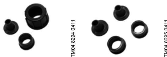
Fig. 45 Left: pump connection kit; right: inlay kit
