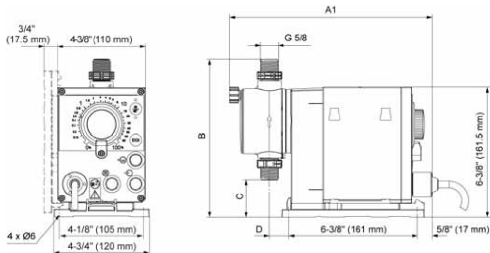
Fig. 22 DDE-PR with front-fitted control elements
