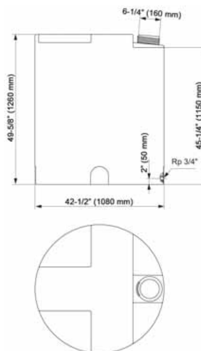
Fig. 52 Cylindrical tank, 264 gal. [1000L]
