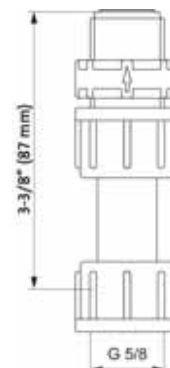
Fig. 44 Pressure valve
