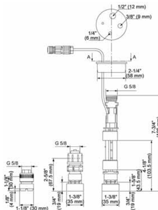
Fig. 31 Left: stainless-steel foot valve; center and right: PE or PVDF foot valve, dimensions
