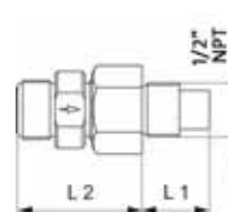
Fig. 35 Standard injection unit, stainless-steel version
