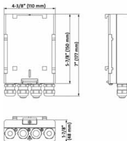
Fig. 28 E-box, dimensions
