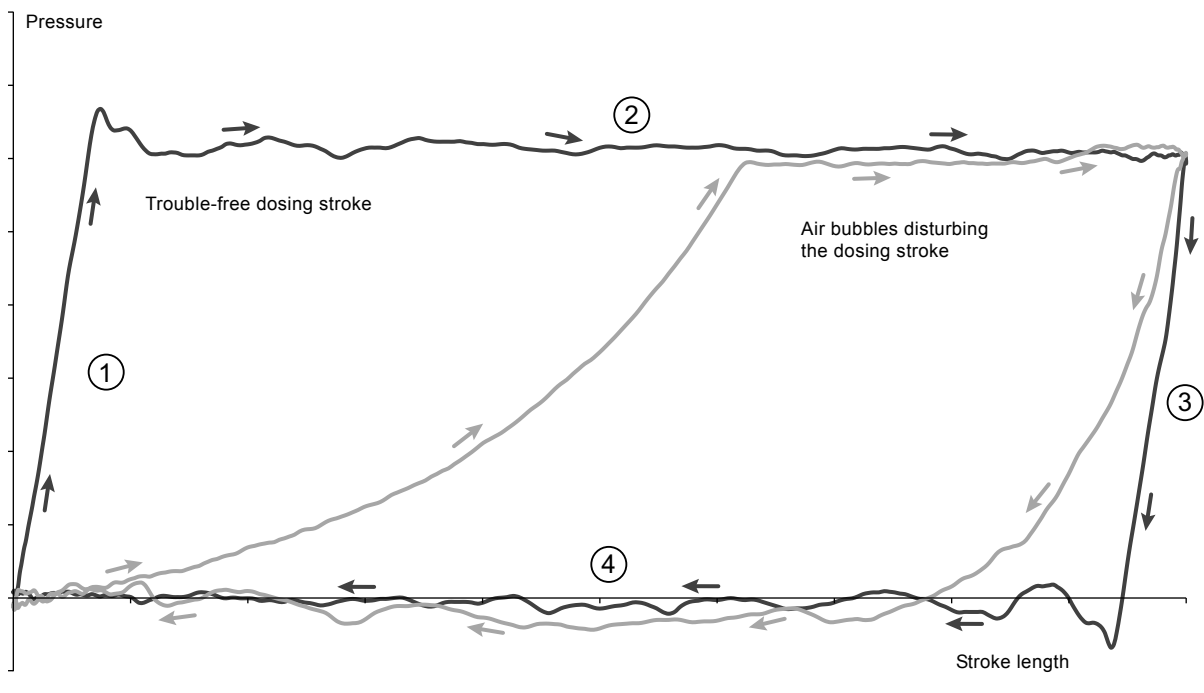
Fig. 18 Indicator diagram
