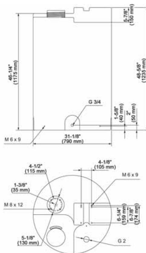
Fig. 51 Cylindrical tank, 132 gal. [500L]
